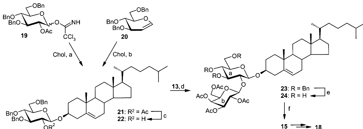
Scheme 2. Synthesis of cholesteryl disaccharide 15 . Reagents and conditions: (a) TMSOTf (0.05 equiv.), CH 2 Cl 2 (88%); (b) DMDO, CH 2 Cl 2 ; ZnCl 2 THF (42%); (c) NaOH, MeOH/dioxane (qu); (d) TMSOTf (0.03 equiv.), IP, CH 2 Cl 2 , room temp. (76%); (e) Pd/C, H 2 , EtOH/CH 2 Cl 2 (qu) or Pd(OH) 2 /C, H 2 , EtOH/dioxane (92%); (f) Ph-CH(OMe) 2 , CSA, MeCN (72%).
