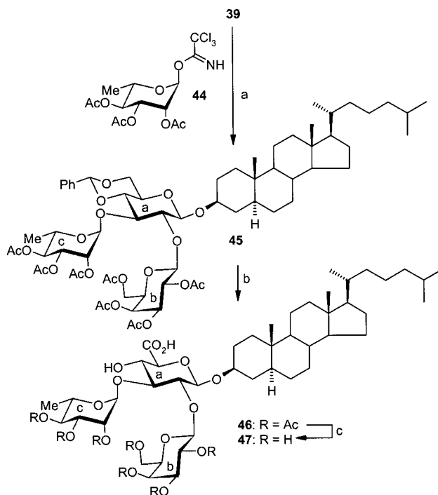
Scheme 6. Synthesis of structural analog 47 . Reagents and conditions: (a) TMSOTf (0.01 equiv.), CH 2 Cl 2 (94%); (b) EtSH, TsOH, CH 2 Cl 2 (88%); TEMPO, NaOCl, TBABr, KBr, CH 2 Cl 2 , NaOH, NaHCO 3 (73%); (c) NaOMe, MeOH/CH 2 Cl 2 , IR-120 (H + ) (95%).
