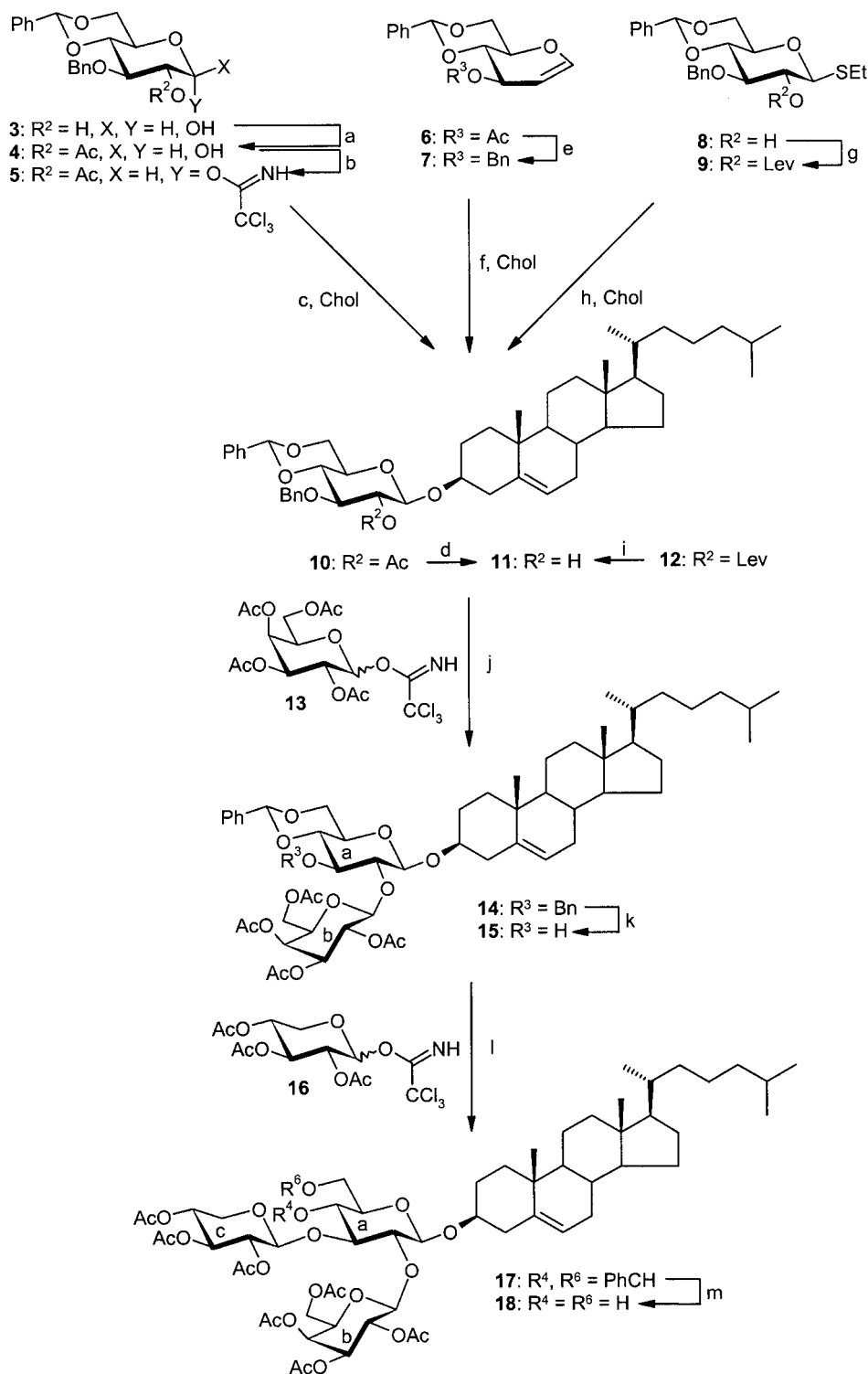
Scheme 1. Synthesis of cholesteryl saccharides 15 and 18 . Reagents and conditions: (a) Ac_2O , Pyr; N_2H_4 \cdot HOAc , DMF (51%); (b) CCl_3CN , DBU, CH_2Cl_2 (73%); (c) TMSOTf (0.05 equiv.), CH_2Cl_2 (41%); (d) NaOMe, MeOH/ CH_2Cl_2 (qu); (e) NaOMe, MeOH; BnBr, NaH, DMF (51%); (f) DMDO, CH_2Cl_2 ; ZnCl 2 , THF (13%); (g) LevOH, DCC, DMAP, CH_2Cl_2 (83%); (h) DMTST, 4-Å mol. sieves, CH_2Cl_2 (68%); (i) N_2H_4 \cdot HOAc , MeOH/ CH_2Cl_2 (80%); (j) TMSOTf (0.05 equiv.), I. P., CH_2Cl_2 (69%); (k) Pd/C, H_2 , EtOH/ CH_2Cl_2 (22%); (l) TMSOTf (0.03 equiv.), CH_2Cl_2 (71%); (m) EtSH, TsOH, CH_2Cl_2 (86%).
