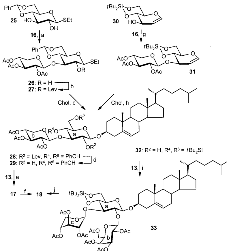
Scheme 3. Synthesis of cholesteryl trisaccharide 18 via a partially convergent route. Reagents and conditions: (a) TMSOTf (0.005 equiv.), 3-Å mol. sieves, IP, -75 → -65 °C, CH 2 Cl 2 (86%); (b) Lev 2 O, NEt 3 , DMAP, CH 2 Cl 2 (94%); (c) DMTST (3 equiv.), 4-Å mol. sieves, CH 2 Cl 2 , room temp. (74%); (d) N 2 H 4 ·HOAc, MeOH/CH 2 Cl 2 (64%); (e) TMSOTf (0.05 equiv.), IP, CH 2 Cl 2 , room temp. (64%); (f) see Scheme 1; (g) TMSOTf (0.001 equiv.), CH 2 Cl 2 , -70 → -45 °C (66%); (h) DMDO, CH 2 Cl 2 , 0 °C → room temp.; ZnCl 2 , THF, -60 °C → room temp. (46%); (i) TMSOTf (0.03 equiv.), I. P., CH 2 Cl 2 , room temp. (91%); (j) HF·Pyr, THF (94%).
